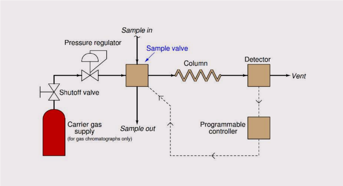
The Gas Chromatography technique
