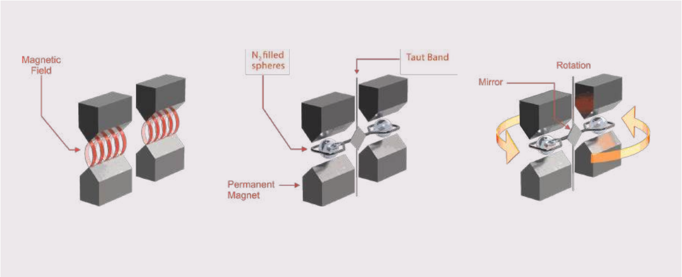
Inside a Paramagnetic cell
