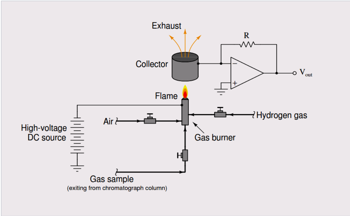
A typical Flame Ionization Detector
