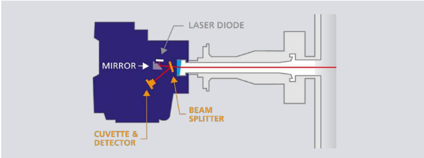
Fig. 1: Close-up of the line lock system showing the cuvette and beam splitter
