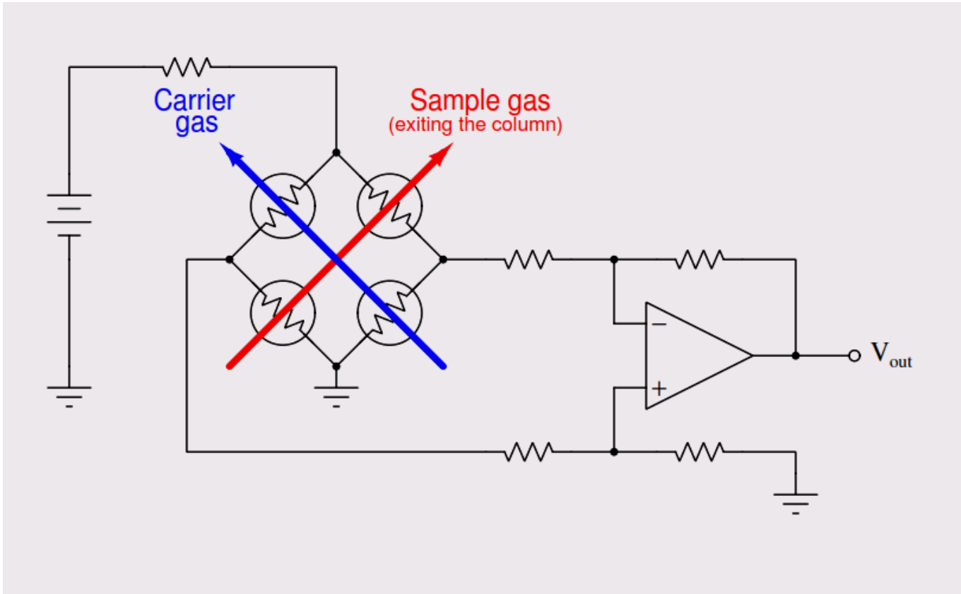
The Thermal Conductivity sensor
