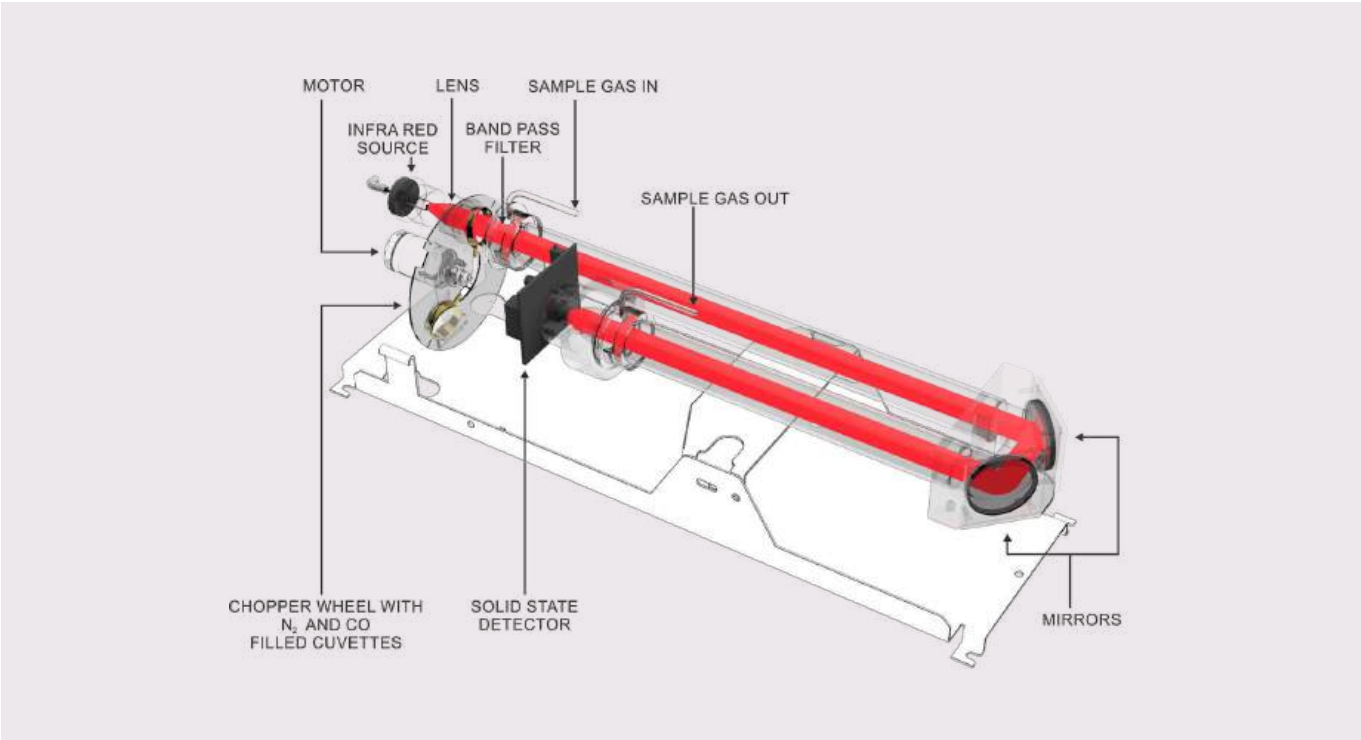
The GFC Transducer
