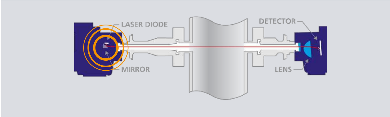
Fig. 2: The SERVOTOUGH Laser 3 Plus installed across a stack, with line lock system (circled)
