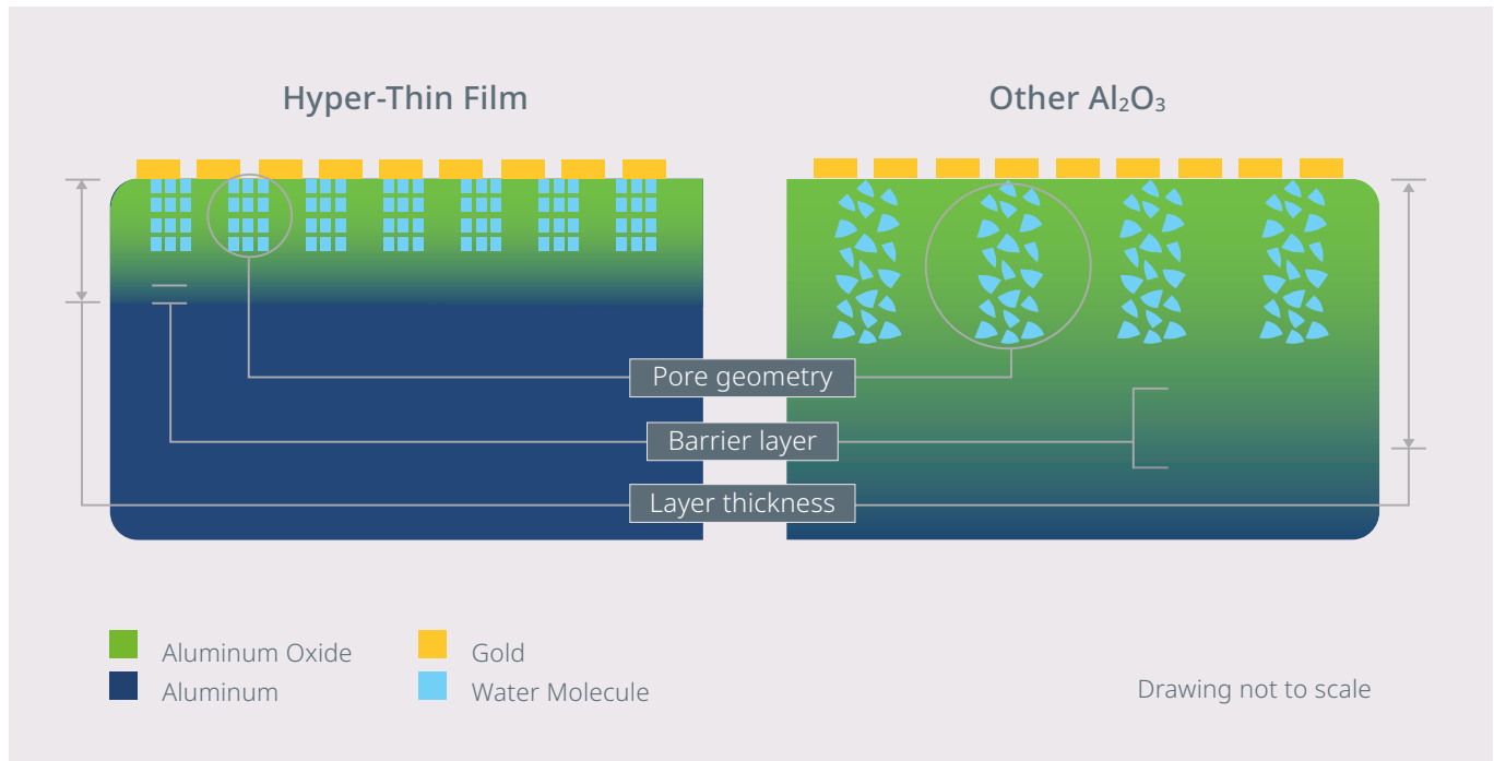
Aluminum Oxide sensor structure
