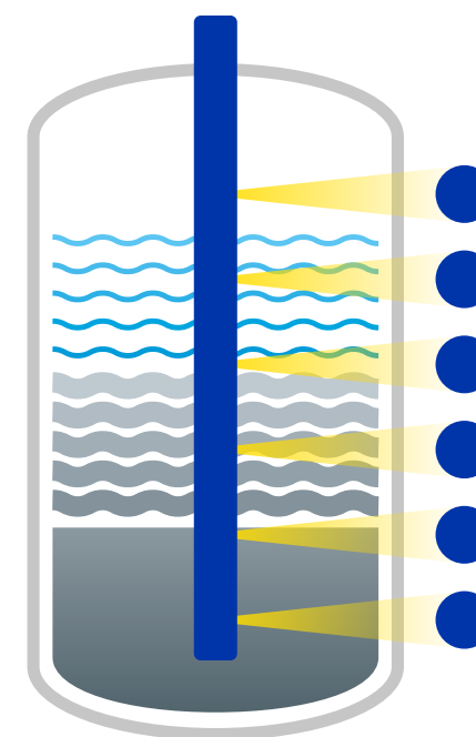
Multiple point sources inserted in dip pipe and density detectors mounted outside the reactor
