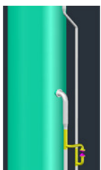
New bypass line between diesel draw-off line to side stripper, new bypass valve, incl. update of P&ID, piping isometrics and pipe stress analysis
