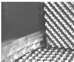
High efficiency Mellapak™ for diesel pumparound
