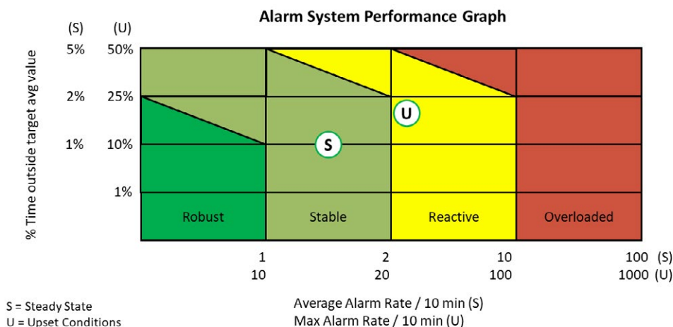
Figure 6: Alarm Performance Graph adapted from EEMUA 191
