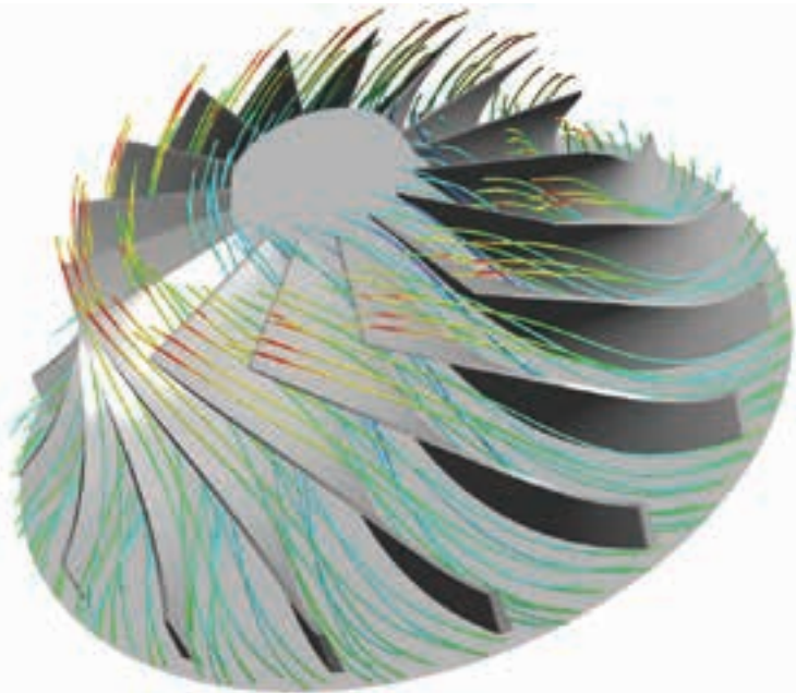
An aerodynamic impeller calculation in CFD
