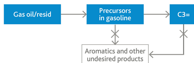
Figure 1: The reactions involved in propylene formation
