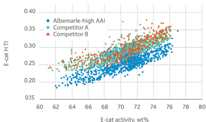
Figure 2: AFX catalysts reduce hydrogen transfer reactions by employing Ketjen's high accessibility technology
