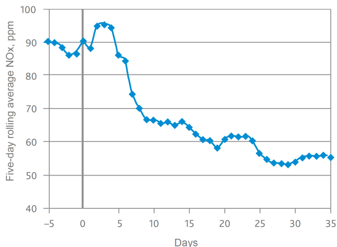
Figure 2: ELIMINOx reduced NOx emissions by 40% at constant afterburn control.
