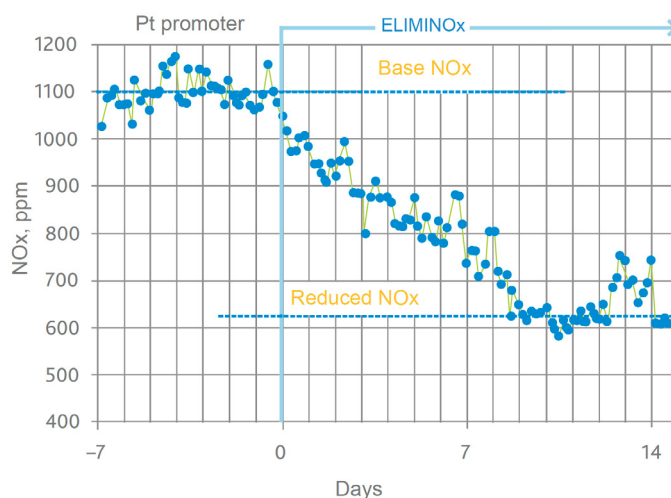
Figure 1: The reduction in NOx emissions by using ELIMINOx can be up to 70%. The 40% NOx reduction shown is typical.
