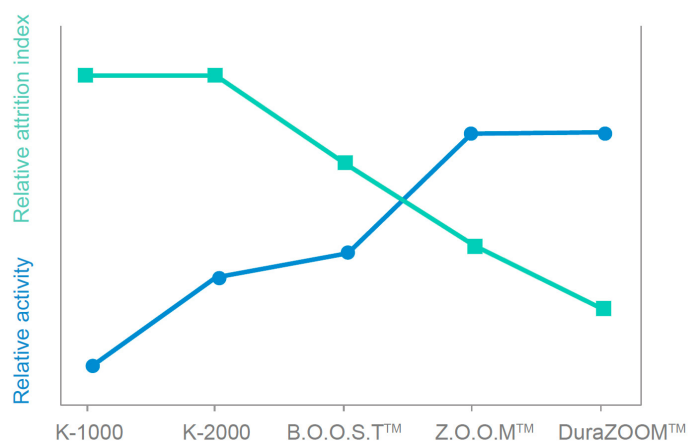
Figure 3: Progressive improvements in activity and attrition resistance over the generations of Ketjen olefin/octane additives
